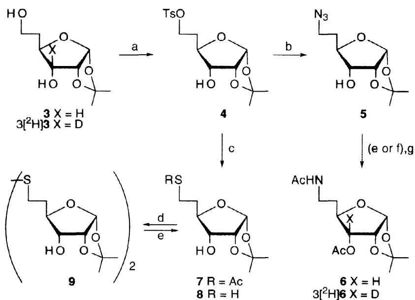
Scheme 2 a
