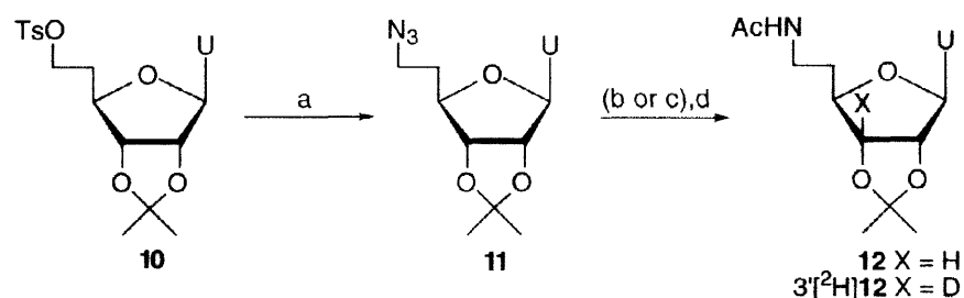
Scheme 3 a
