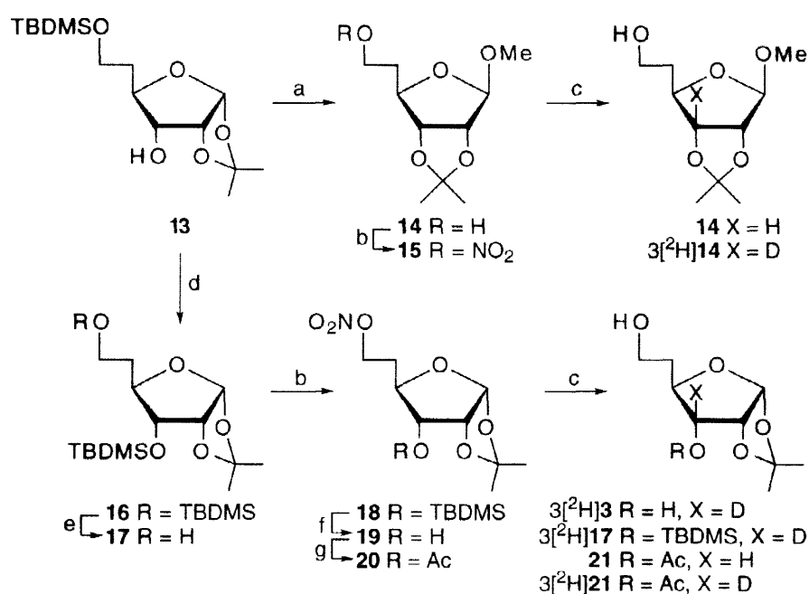
Scheme 4 a
